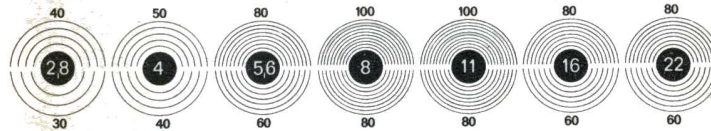
Planar 2,8/80 mm.
